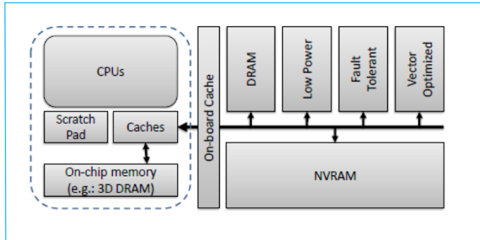
Simplified view of a heterogeneous memory node sample. 4
