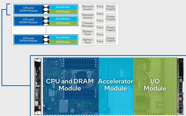
1-Socket Disaggregated Server Example
