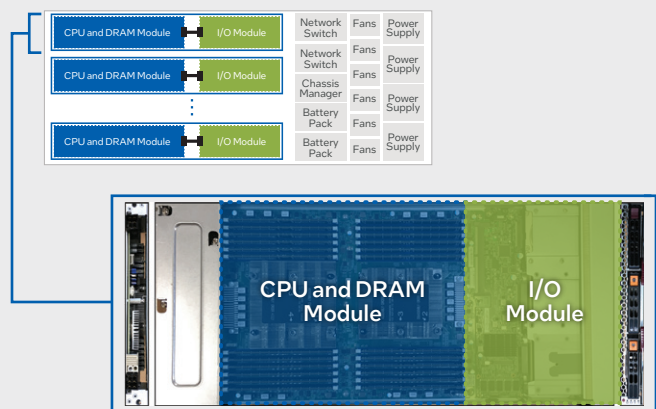
2-Socket Disaggregated Server Example
